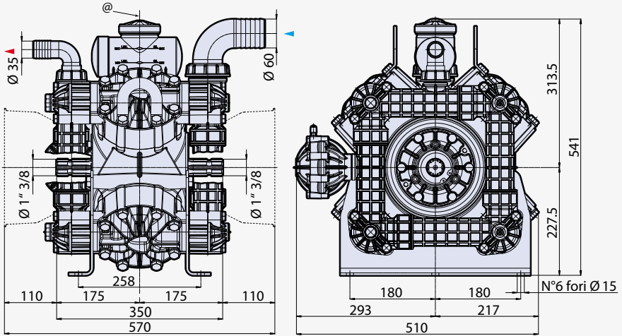
@ = Pump axis - Asse pompa
